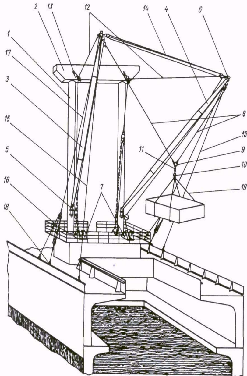
Fig. 4 Typical rigging for union purchase
