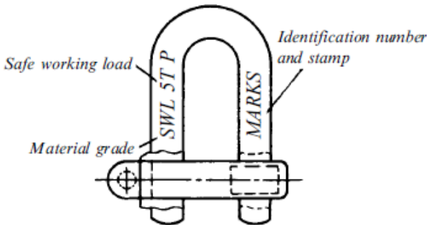
Fig. 11.2.1.2. Marking of shackles
