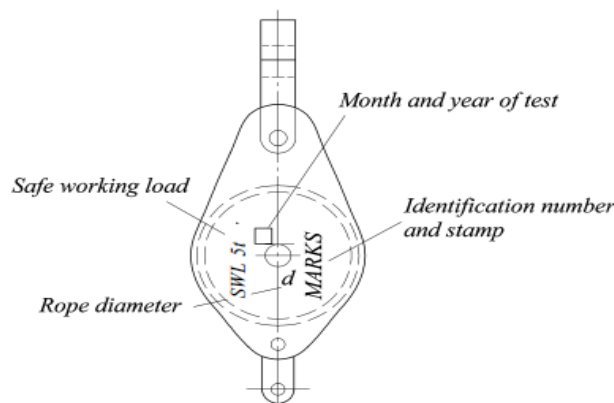
Fig. 11.2.1.5. Marking of blocks
