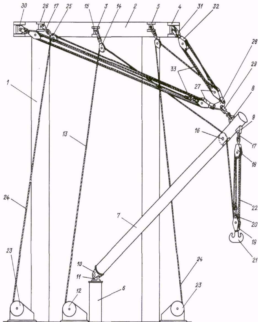
Fig. 3 Typical rigging of twin span tackle heavy-lift derrick
