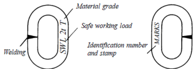
Fig. 11.2.1.4. Marking of chains
