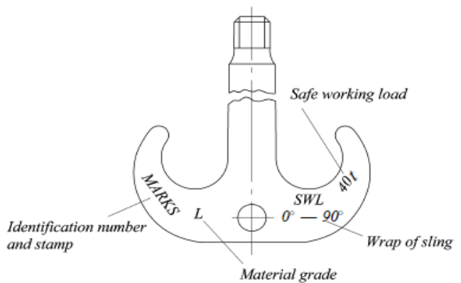
Fig. 11.2.1.3. Marking of ramshorn hooks
