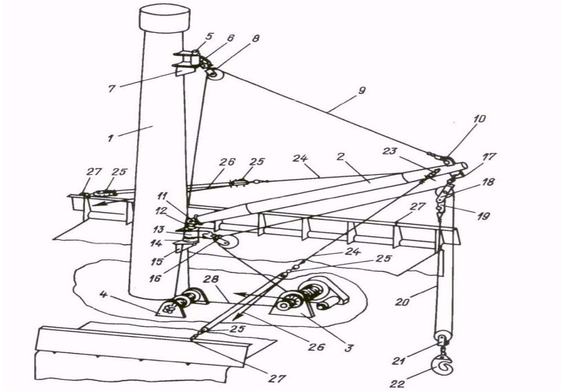
Fig. 1 Typical rigging of light-lift derrick
