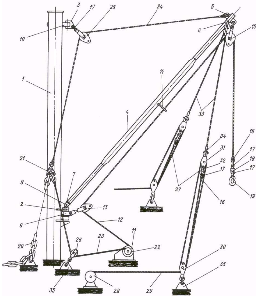
Fig. 2 Alternative rigging of light-lift derrick
