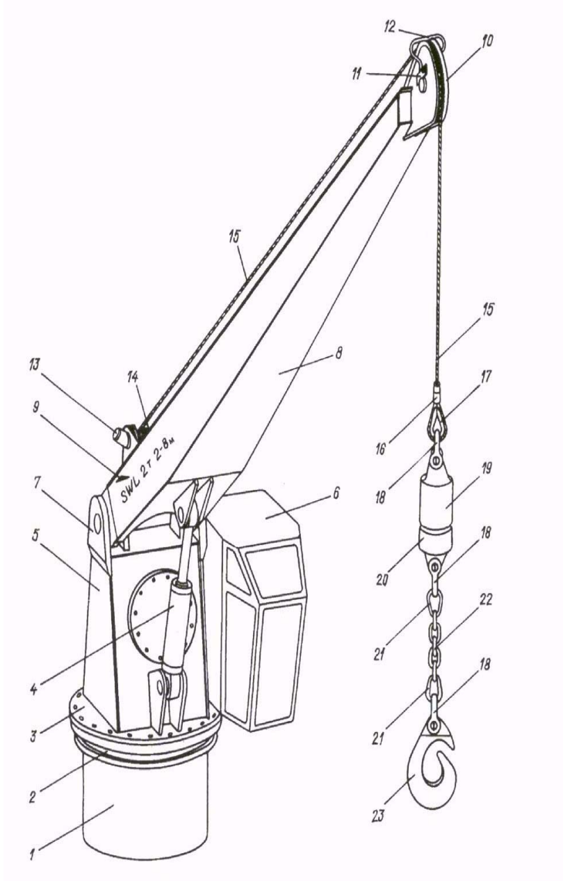
Fig. 5 Deck full-swing crane
